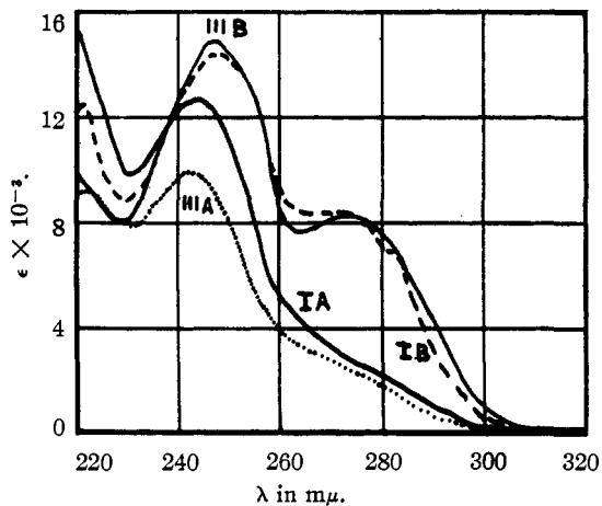
Fig. 1.—Ultraviolet absorption spectra of IA, IB, IIIA and IIIB in heptane.
