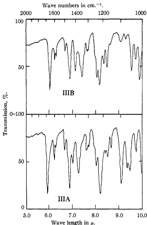
Fig. 9.—Infrared spectra of IIIA and IIIB.
