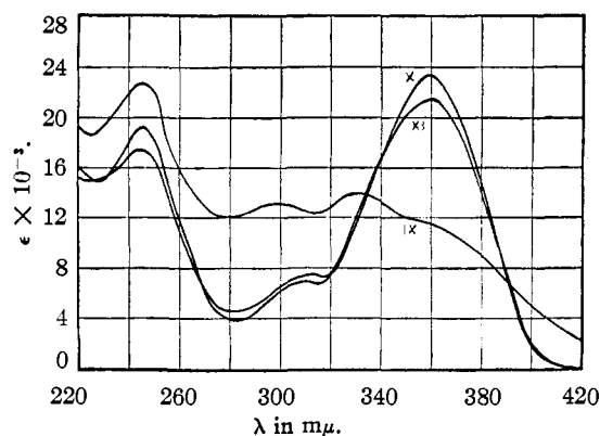
Fig. 5.—Ultraviolet absorption spectra of IX in ethanol and X and XI in heptane.
