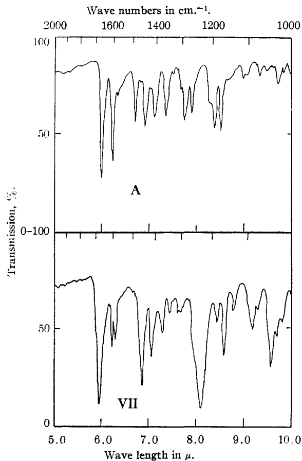
Fig. 12.—Infrared spectra of VII and A (benzyl- p -methylacetophenone).
